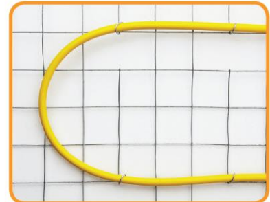
3261 In Screed Cable Mesh
